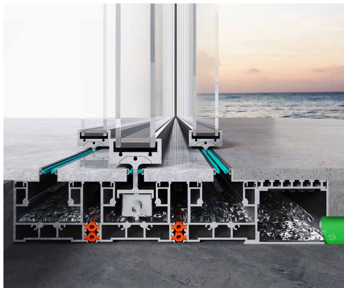
TRACK AND GLAZING SECTION
